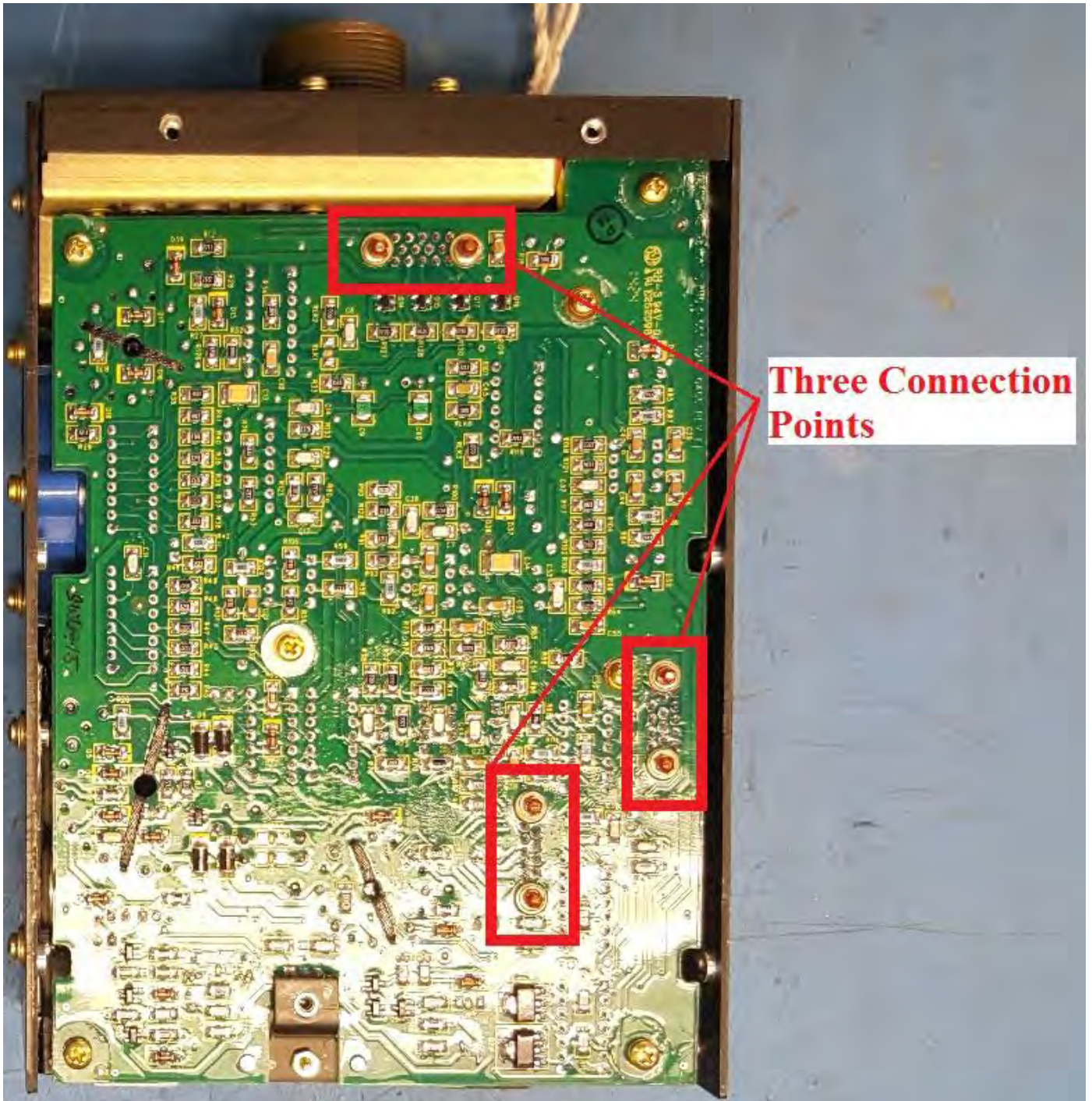
Figure 3 – PCB view (Connection Points Before Removal)
