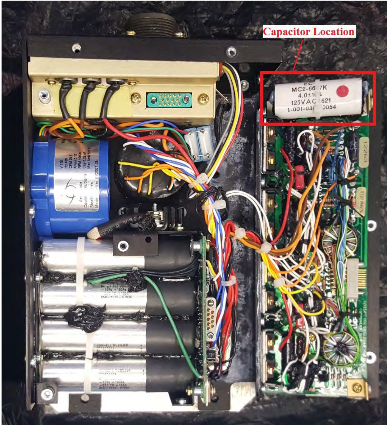
Figure 6 – Interior/Bridge Assembly View (Capacitor Location)
