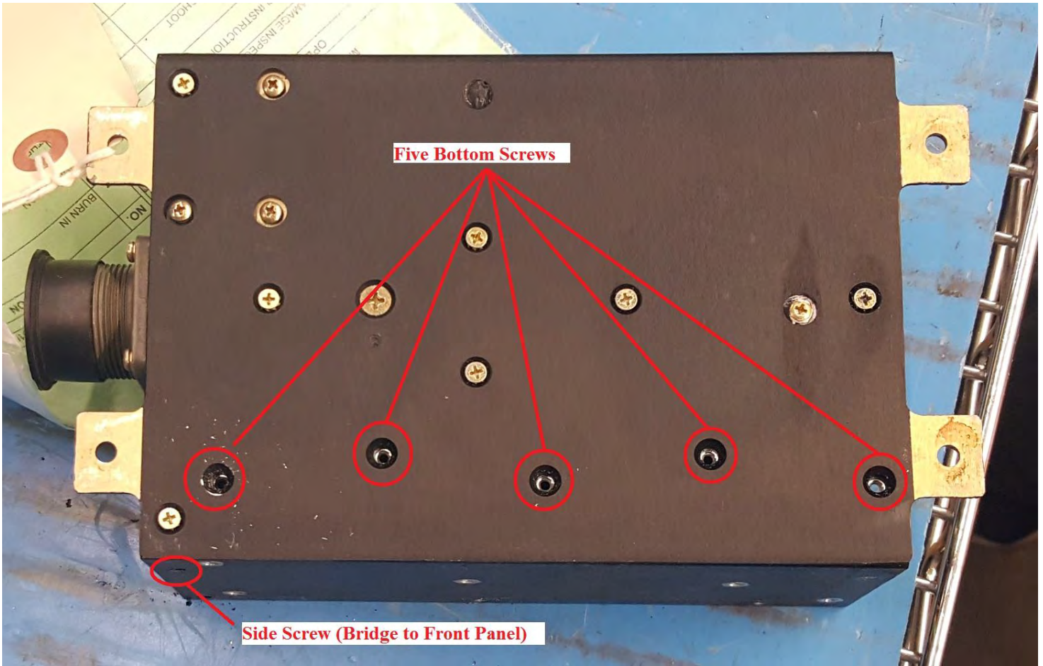
Figure 5 - Bottom view (Bottom Screw Locations, Side Screw Location)
